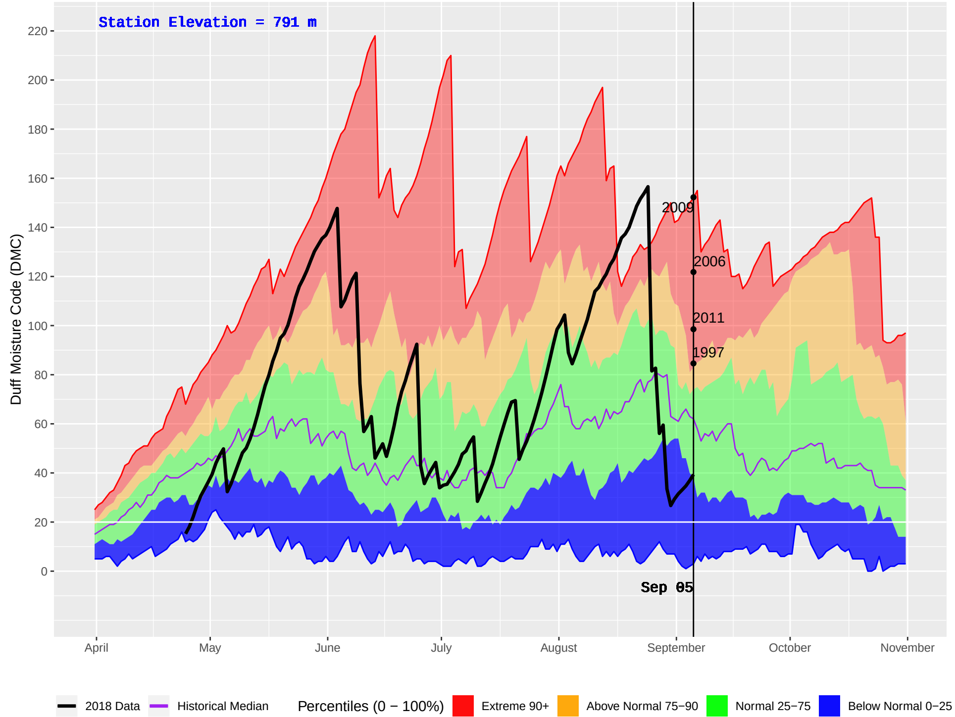
ALEXIS CREEK (209) : Historical (1980–2016) and Current (2018) Daily Duff Moisture Code (DMC)
